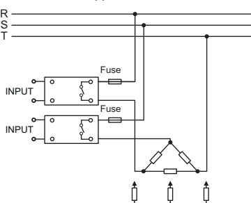
Three Phase Load Application With The Two SSRs
