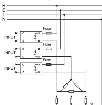
Three Phase Load Application With The Three SSRs
